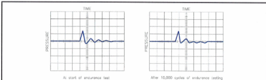
Figure 13: P.D.I. Water hammer arrester
