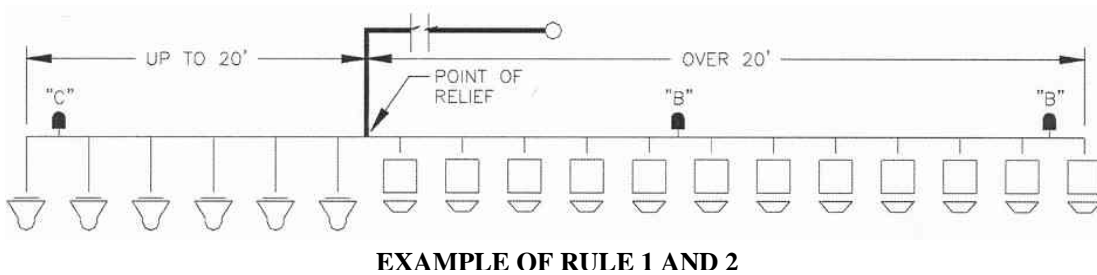
Figure 20: Note: There are practical limits concerning the overall length of a branch line. In a remote instance where a very long line branch line is involved, the general supply is generally fed to some mid-point or other location on the branch line as shown.
