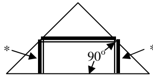
Building Segment More Than 60° to Horizontal - Wall.
